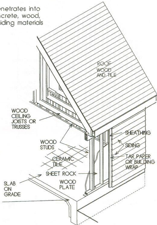
Wood Frame Construction
